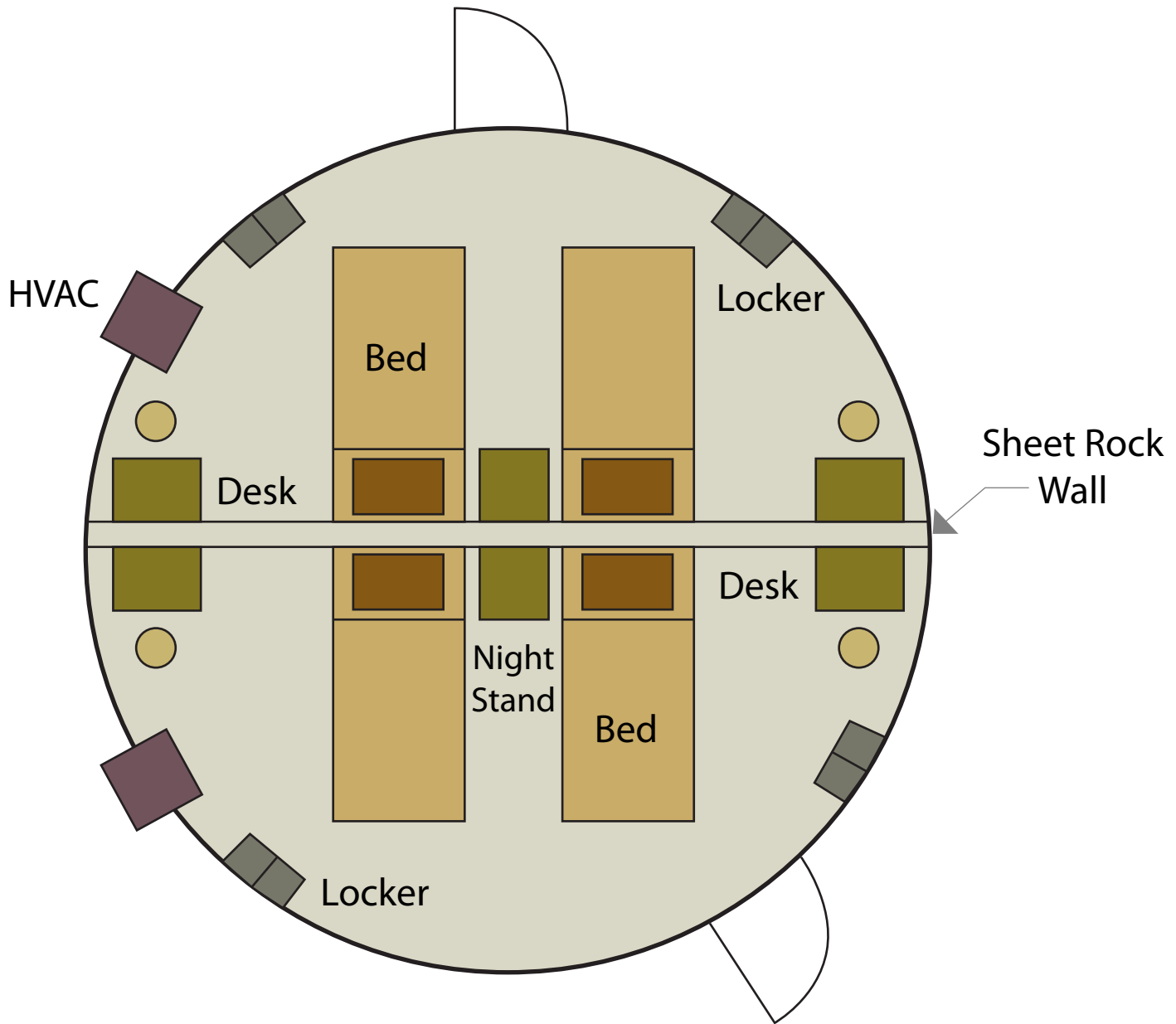
4 Person Layout
